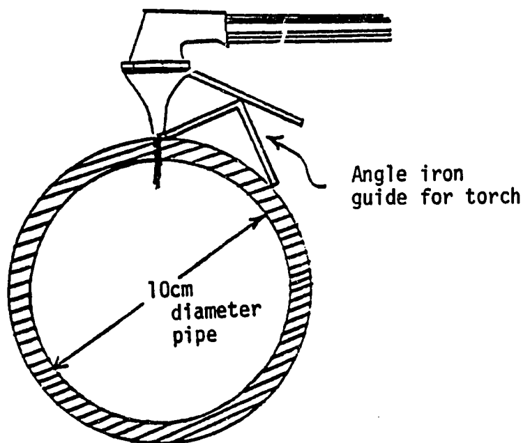
Figure 11. End View
