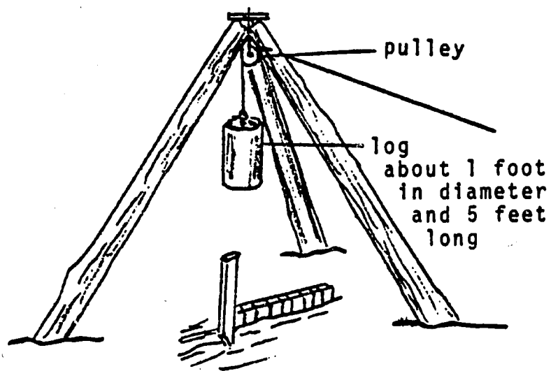
PILE DRIVER
