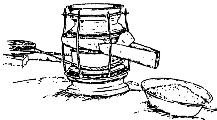
Figure 3. Village Peanut Huller
