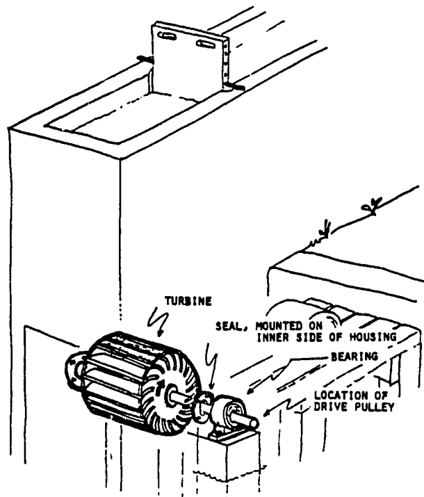
Figure 21. Unobstructed View of The Turbine, Seal and Bearing
