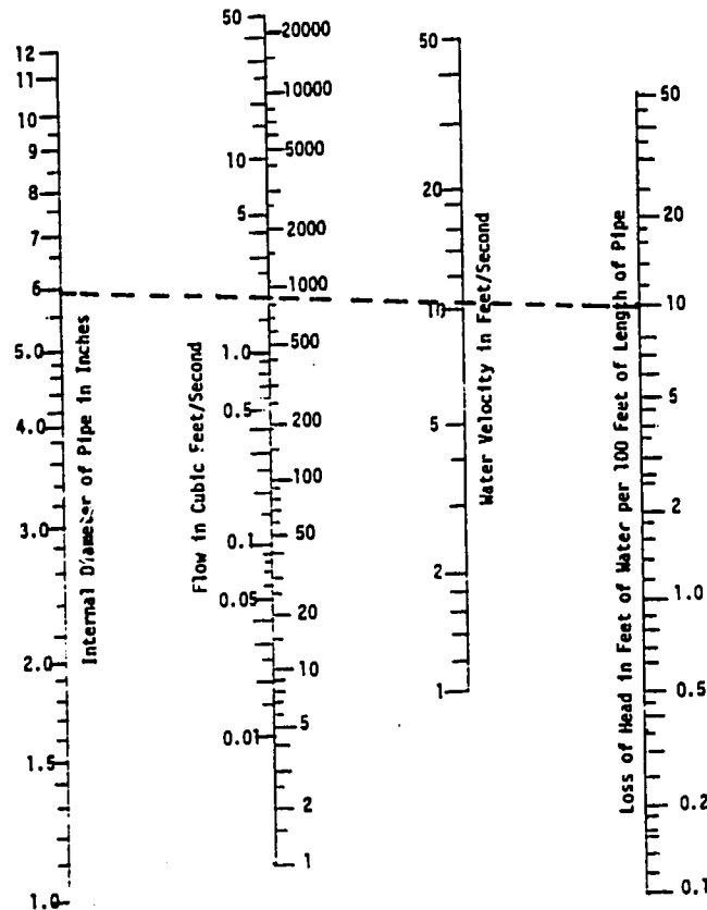
NOMOGRAPH FOR HEAD LOSS IN STEEL PIPES
