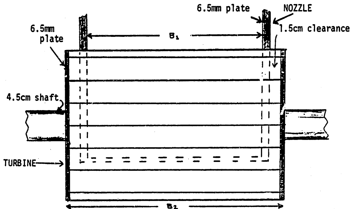
Figure 18. Turbine and Nozzle--Front View
