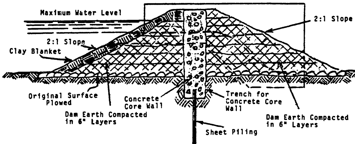
EARTH-FILL DAM
