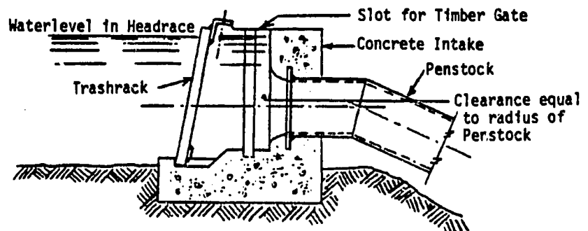
SECTIONAL ELEVATION: INTAKE TO PENSTOCK OF SMALL WATER TURBINE
