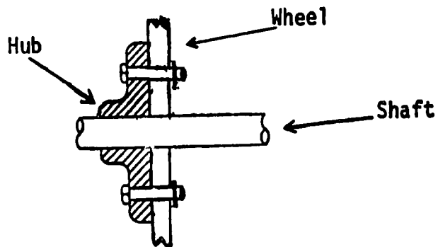
Figure 13. Hub Placement
