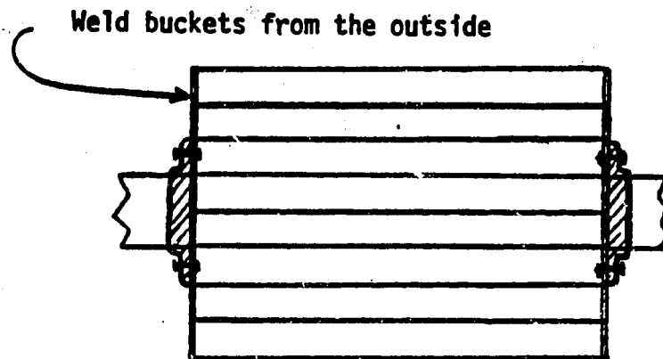
Figure 15. Bucket Placement
