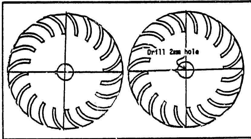
Figure 9. Center Hole
