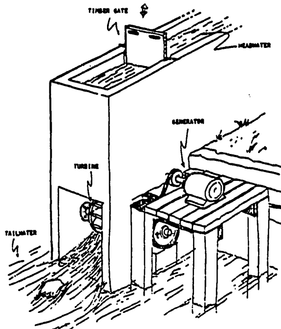
Figure 2. Michell Turbine
