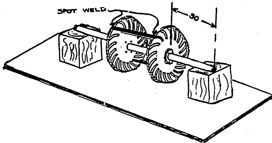
Figure 14. Blade Alignment
