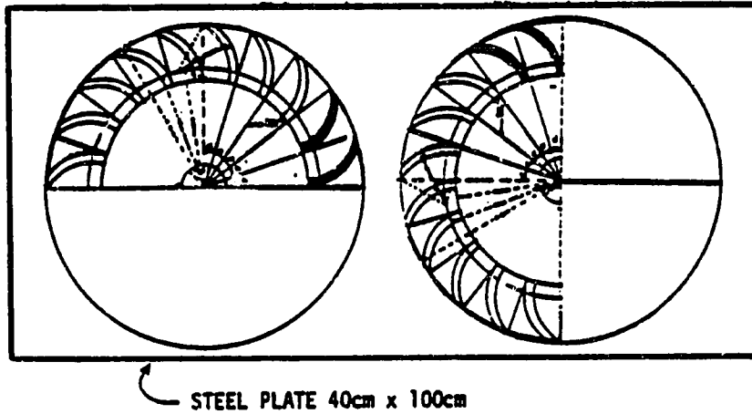
Figure 5. Trace Template on Steel Plate
