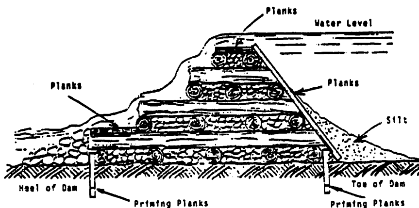
Crib Dam without Downstream Planking
